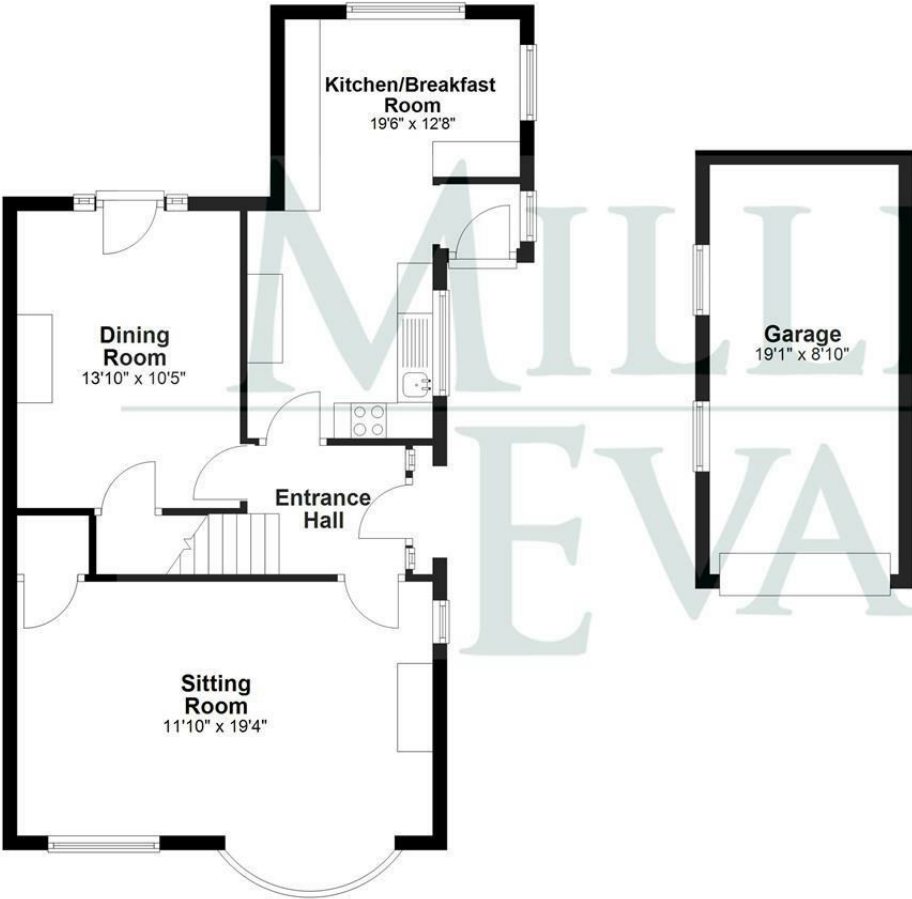
Ground Floor Approx. 838.9 sq. feet
